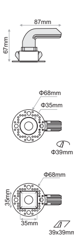
IDC.022 Trimless base for round version IDC.025 Trimless base for square version
